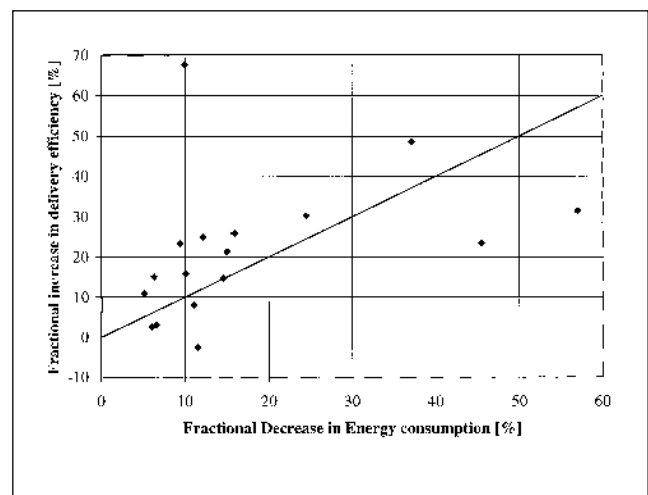
Figure 1. Use of Delivery Efficiency to Predict Reduction in Energy Consumption.
