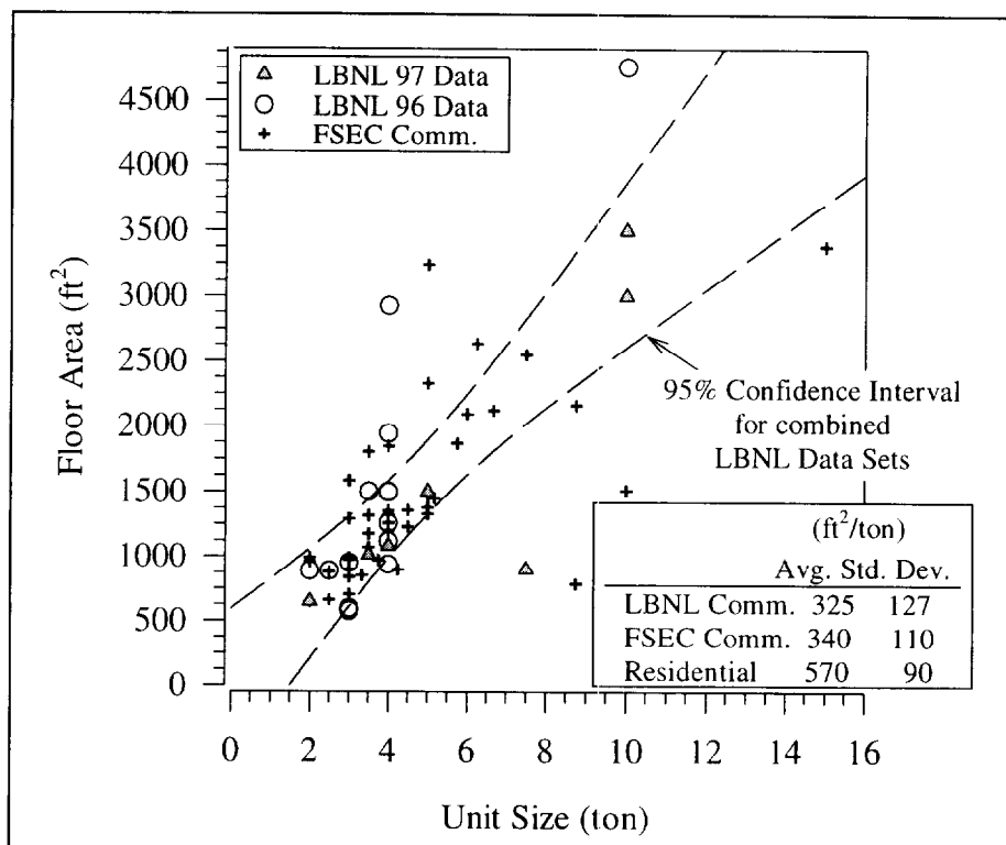
Figure 1. Floor area -vs- unit size: using the 1996 and 1997 LBNL and FSEC (Cummings, et al., 1996) commercial data along with residential (Jump, et al., 1996) summary information. The FSEC unit size is derived from the total installed capacity in the building divided by the number of units.
