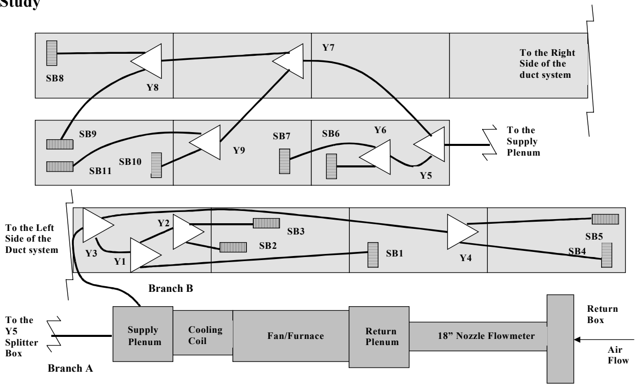
Figure 4. Layout of the Complete Residential Air Distribution System Built for the Study
