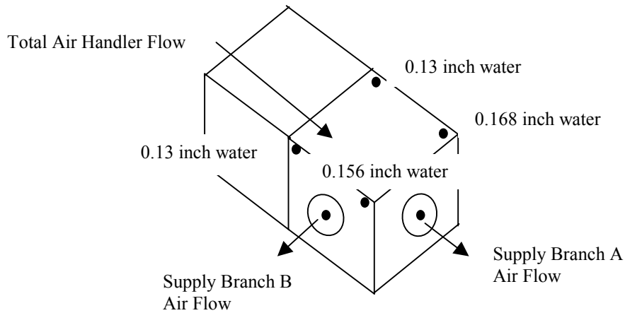
Figure 5. Location of the Measured (Upper Corners) and Calculated (at Entry) Static Pressure Values in the Installed System
