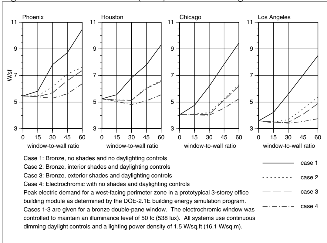
Figure 1. Peak Electric Demand (W/ft 2 ) for a West-Facing Perimeter Zone
