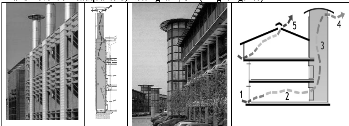
Figure 3. Heat Extraction and Stack Ventilation System in the Environmental Building, Building Research Establishment, Garston, UK (2 left figures) and the Inland Revenue Headquarters, Nottingham, UK (2 right figures)
