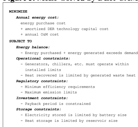
Figure 3. MILP Solved by DER-CAM 6
