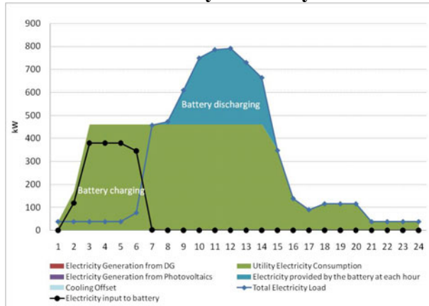
Figure 8. Low Storage and PV Pprice (run 3) Diurnal Electricity Pattern for the School on a May Weekday
