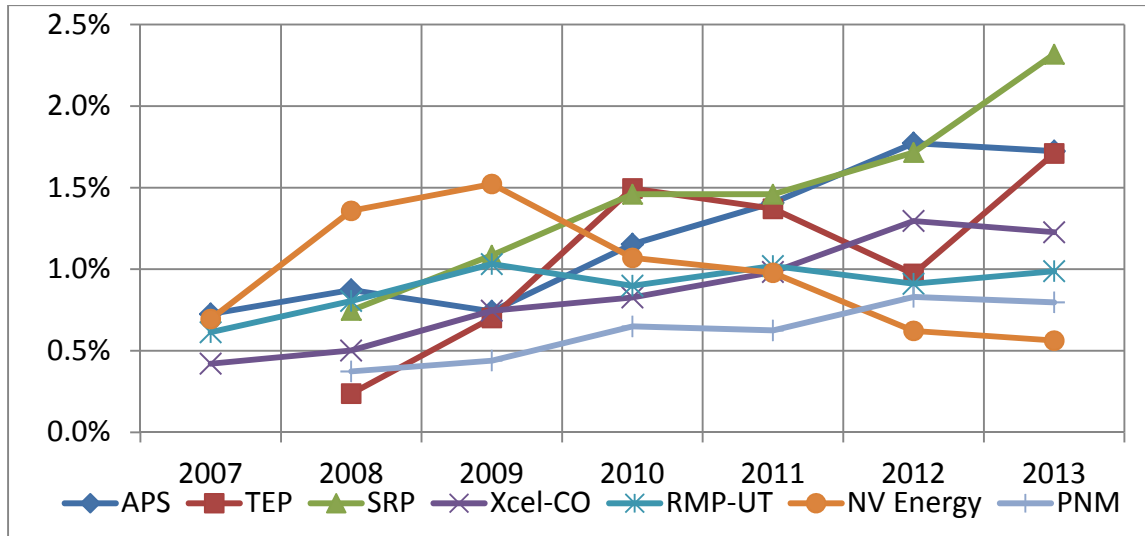
Figure 1. First year energy savings as a fraction of retail electricity sales.
