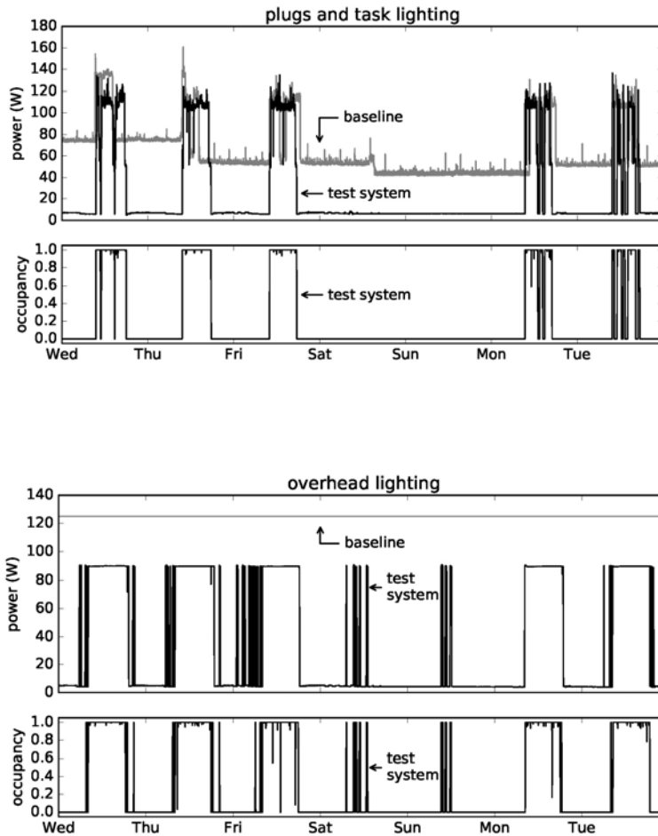
Figure 2. Overhead lighting and plug load operation in response to occupancy for baseline and test cases
