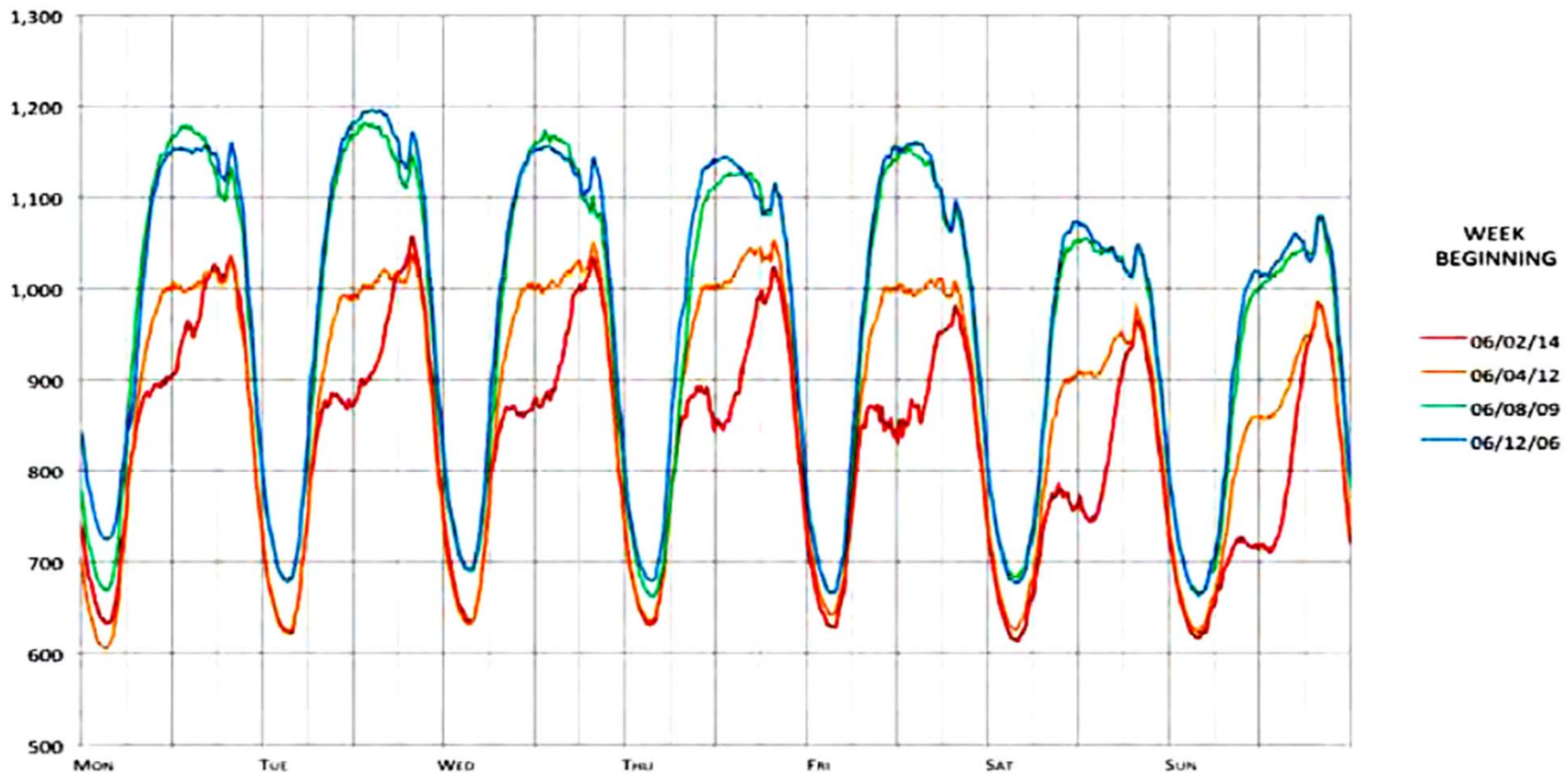
HAWAIIAN ELECTRIC COMPANY, INC. HISTORICAL COMPARISON OF SYSTEM LOAD TYPICAL WEEK IN JUNE
