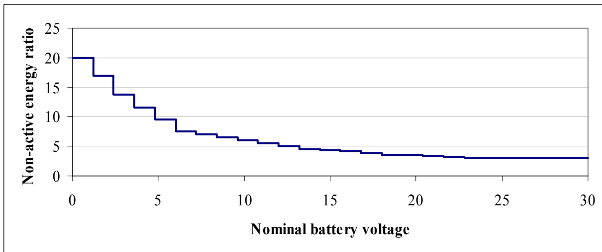
Figure 5. Energy Performance Criteria for Battery Charging Systems
