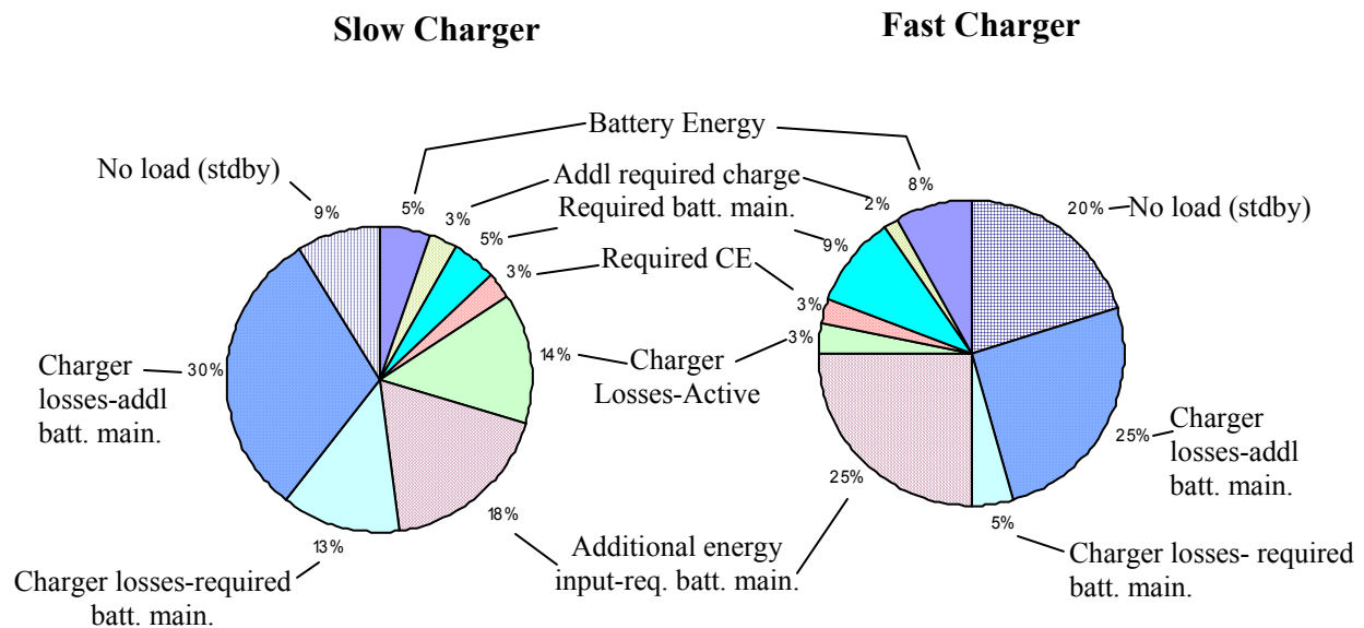
Figure 2. Energy Used in Slow and Fast (1 hour) Chargers for Power Tools
