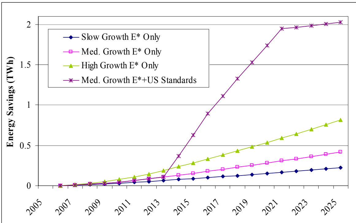
Figure 8. Energy Savings for Battery Charging Systems (TWh)
