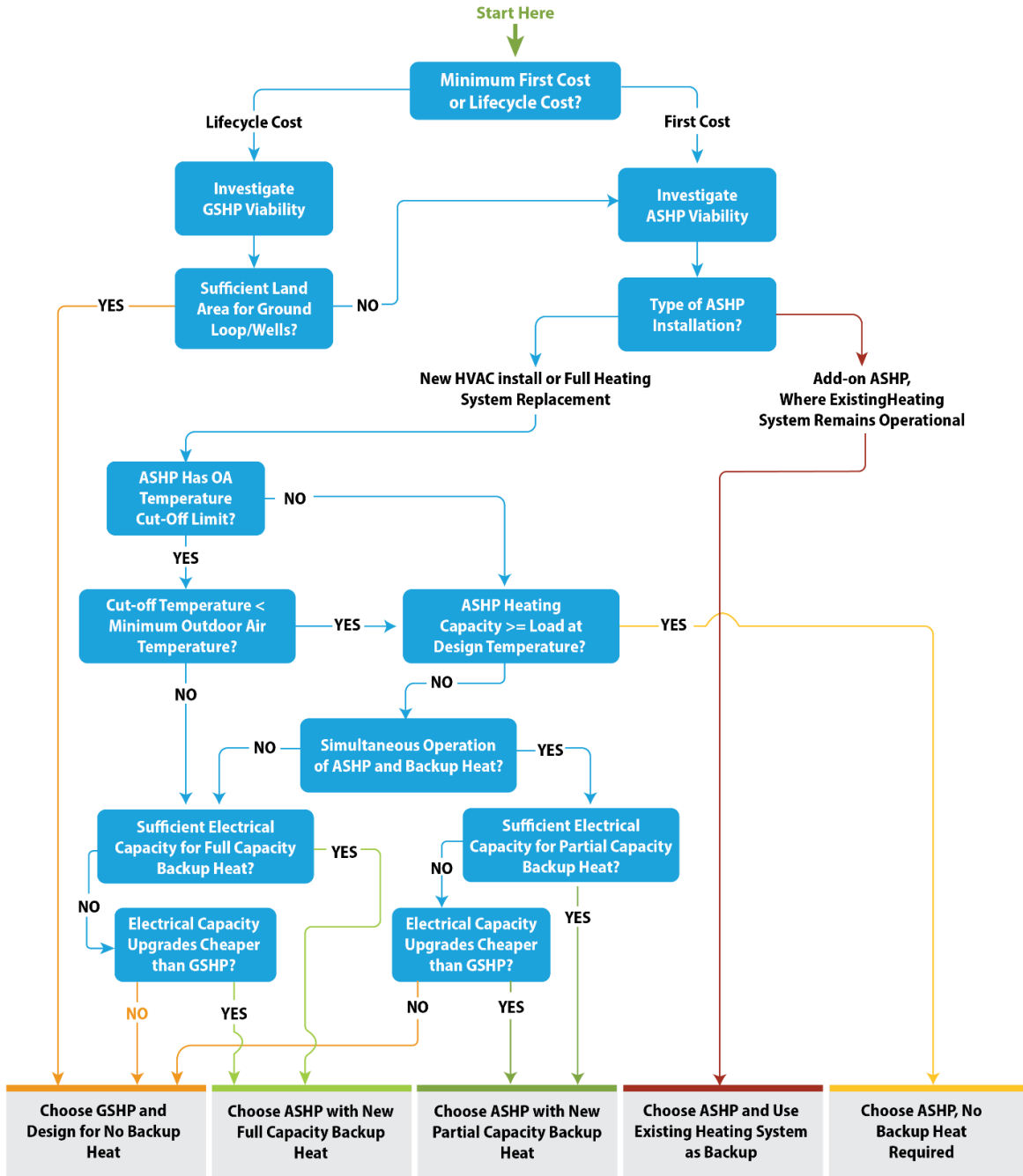
Figure 4. Decision tree to help designers identify backup heat requirements for air-source heat pumps. Source: Houssainy et al. 2024 Key: GSHP: ground-source heat pump; ASHP: air-source heat pump; OA: outside air
